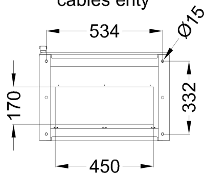
Bottom view ground fixing and cables entry
